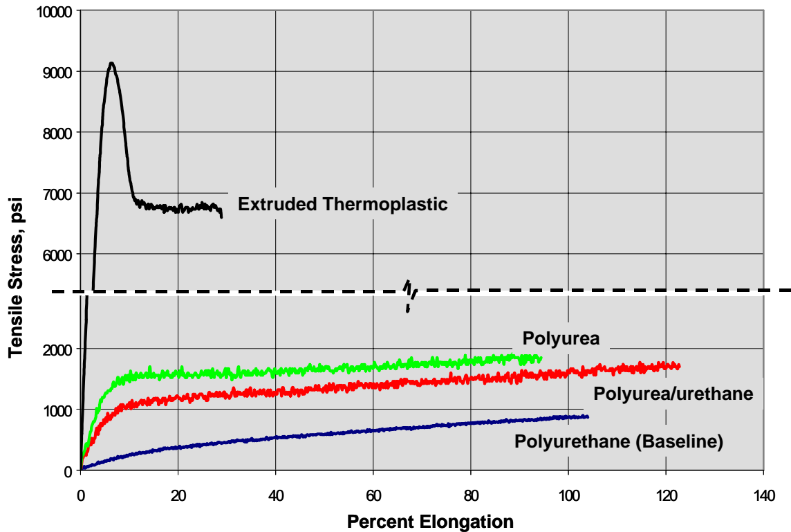
Figure 5. Typical Results from Polymer Tensile Testing
