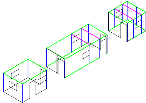
Reinforcement Scheme
