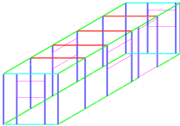
Figure 9. Steel Reinforcement Scheme for Structure 1 Test
