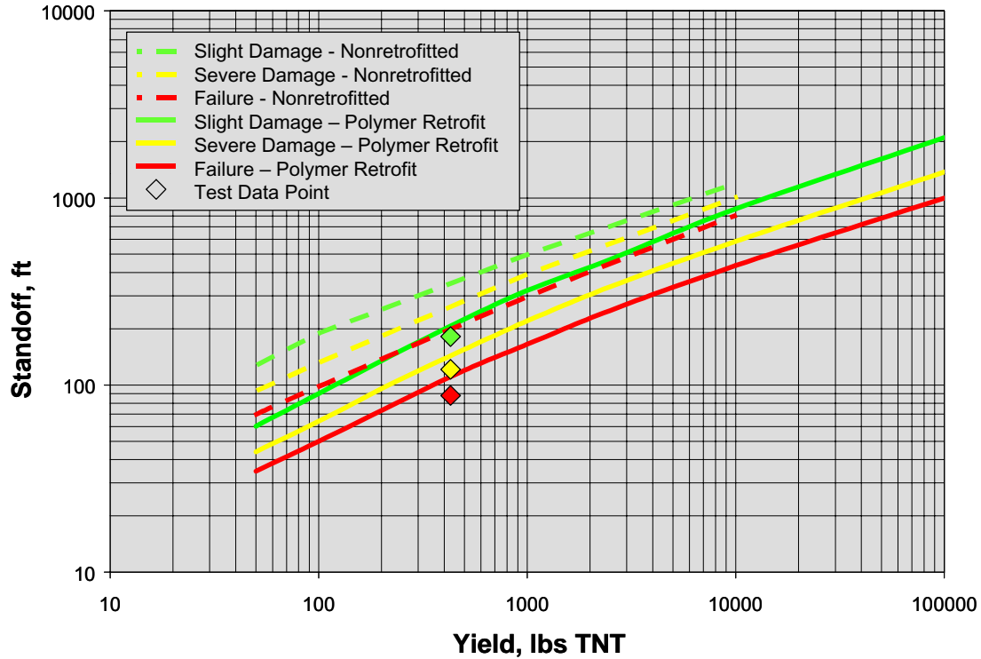
Figure 14. Standoff Curves for Retrofitted and Nonretrofitted Lightweight Structures
