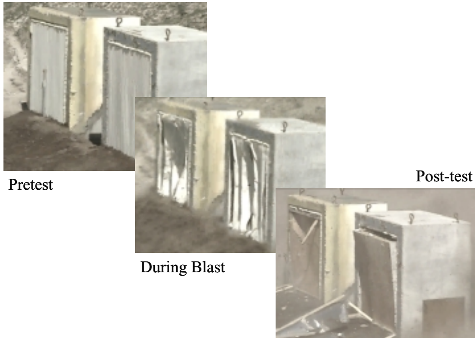
Figure 7. Component Wall Test
