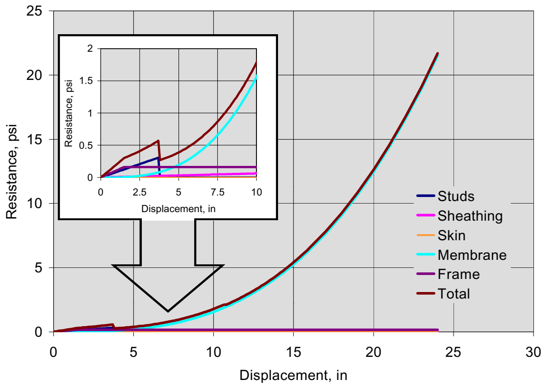
Figure 6. Typical Composite Resistance Function for Lightweight Shelter Wall.
